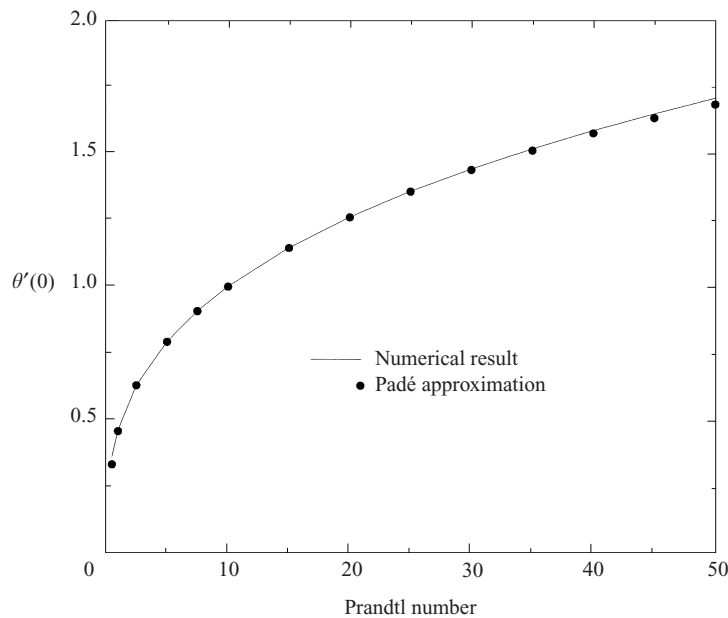
FIGURE 3. Comparisons of numerical results with the Padé expression (3.12) for \theta'(0) for \kappa = 1/2 when \bar{h} = -2/5 .
